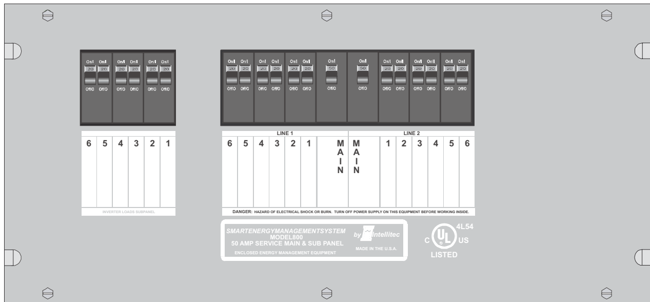
50 Amp EMS MODEL 800 DISTRIBUTION PANEL P/N 00-00683-300
